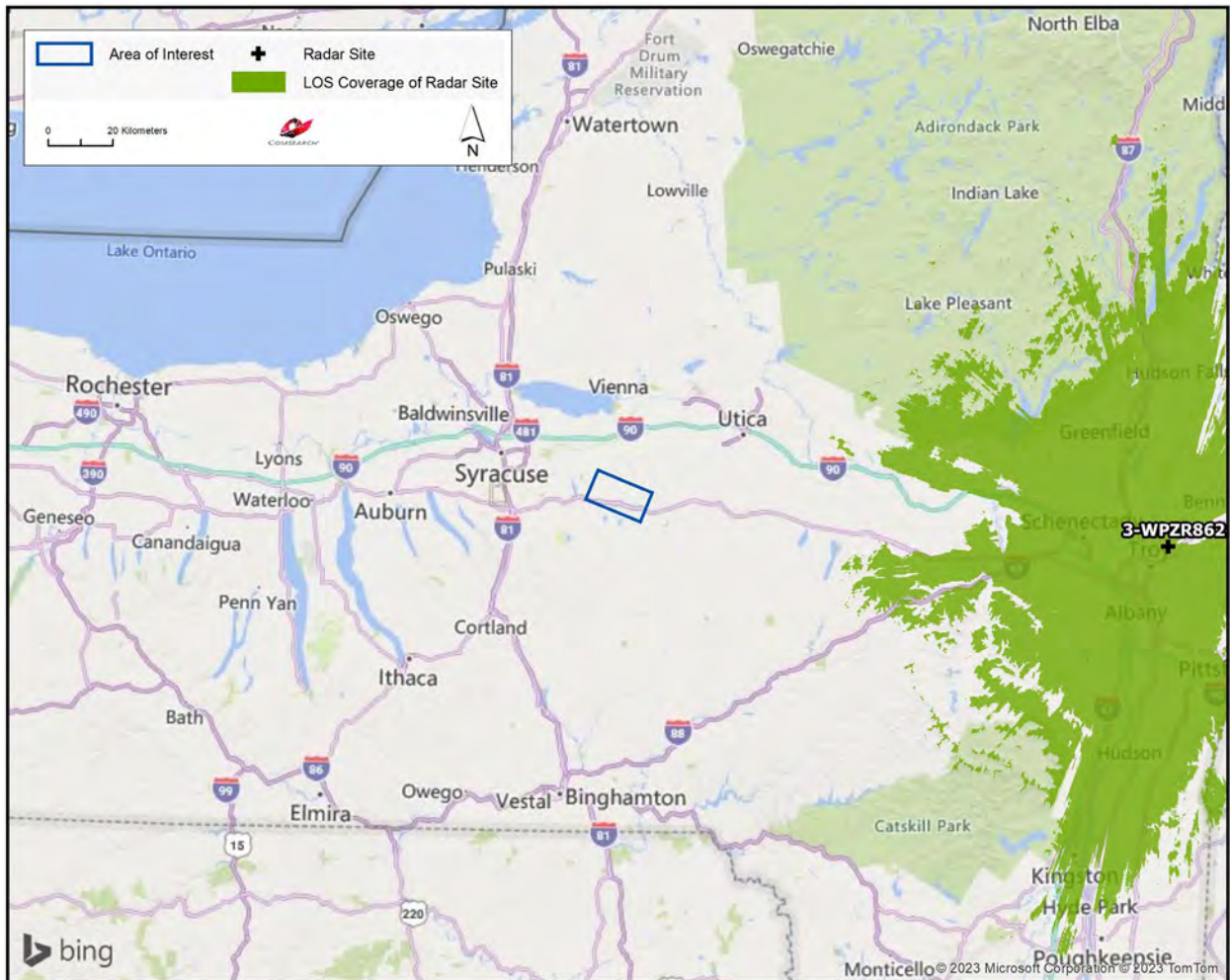
Figure A1-3: Line-of-Sight Coverage of WPZR862 with Respect to Hoffman Falls Project
